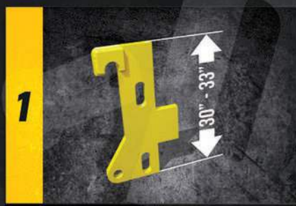
1 SELECT COUPLER HOOKS THAT FIT YOUR MACHINE
